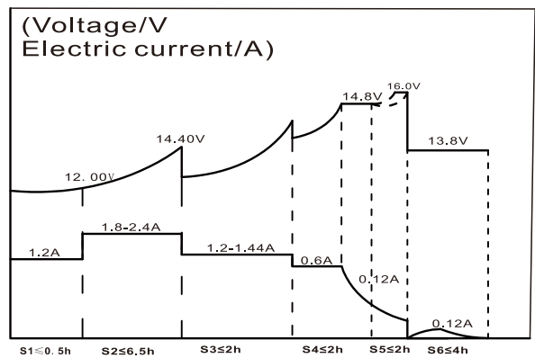
Charging characteristic
