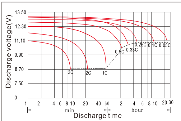
Discharge characteristic
