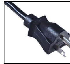
3G x 16AWG x 2m with NEMA5-15P Plug
